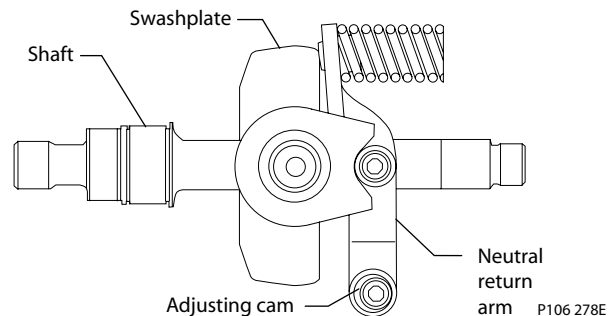
Neutral return mechanism
