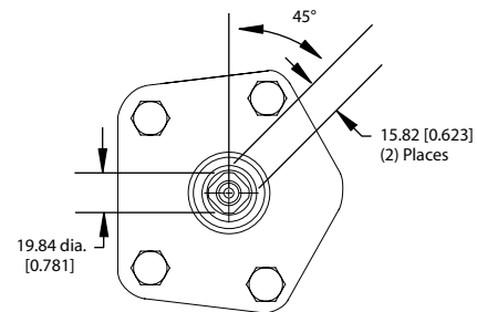
CONTROL TRUNNION DETAIL
